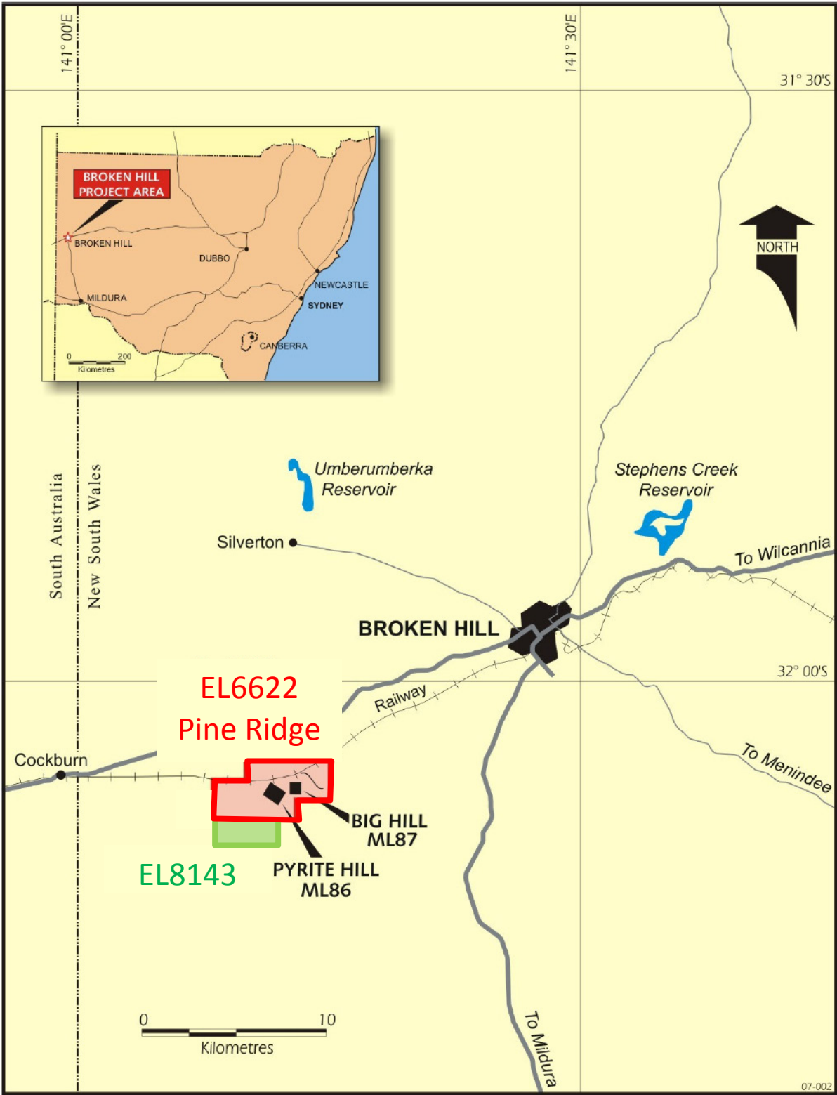
Figure 1. Thackaringa cobalt-pyrite project – Tenements location map.
